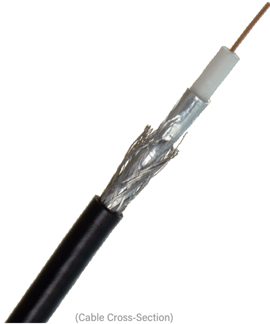
(Cable Cross-Section)
